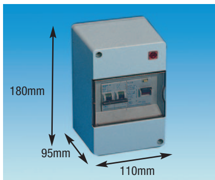
P0103 - Mains Consumer Unit. This unit gives you maximum security with mains electricity in your caravan.
