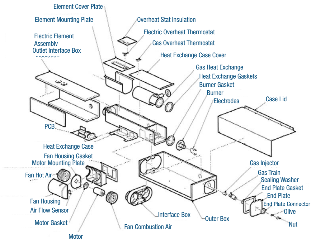
Fig. 1 - Components List
