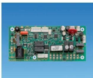
AK1264 - Main PCB (without Reset button 770.215)
