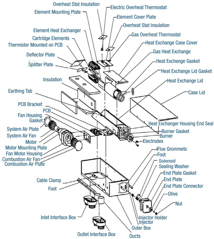
Fig. 1 - Components List
